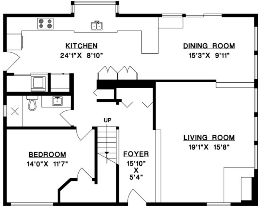
MAIN FLOOR
