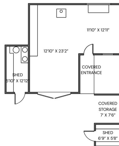
WORKSHOP MAIN LEVEL
