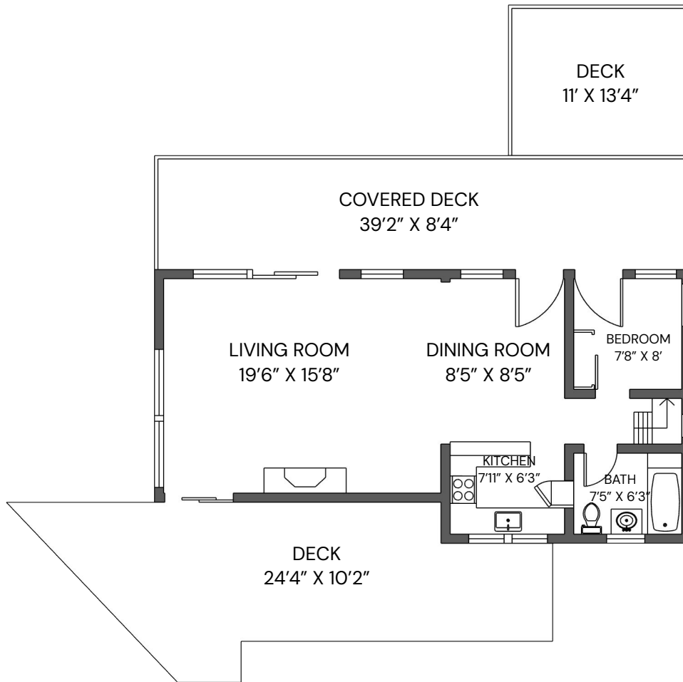
MAIN LEVEL
