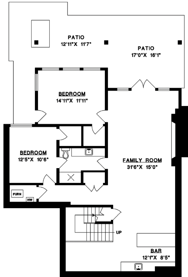
LOWER FLOOR
