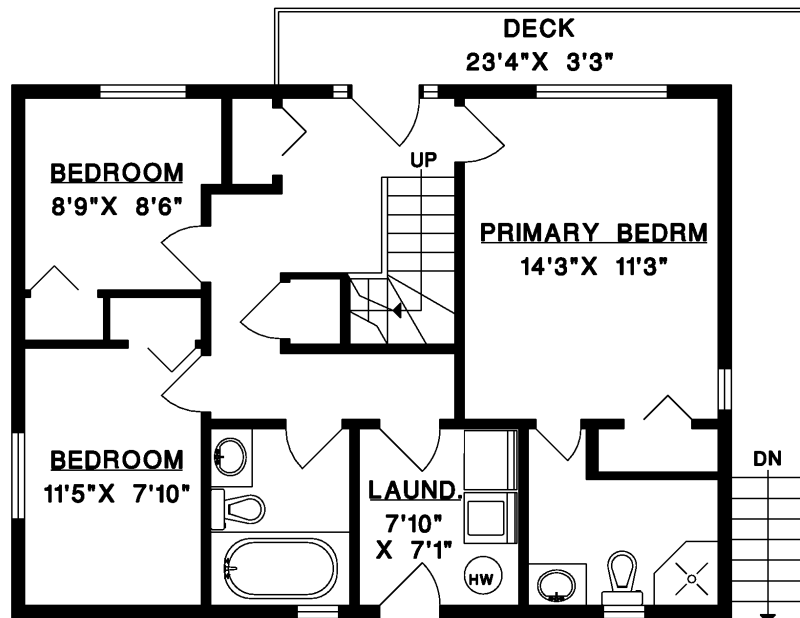
LOWER FLOOR
