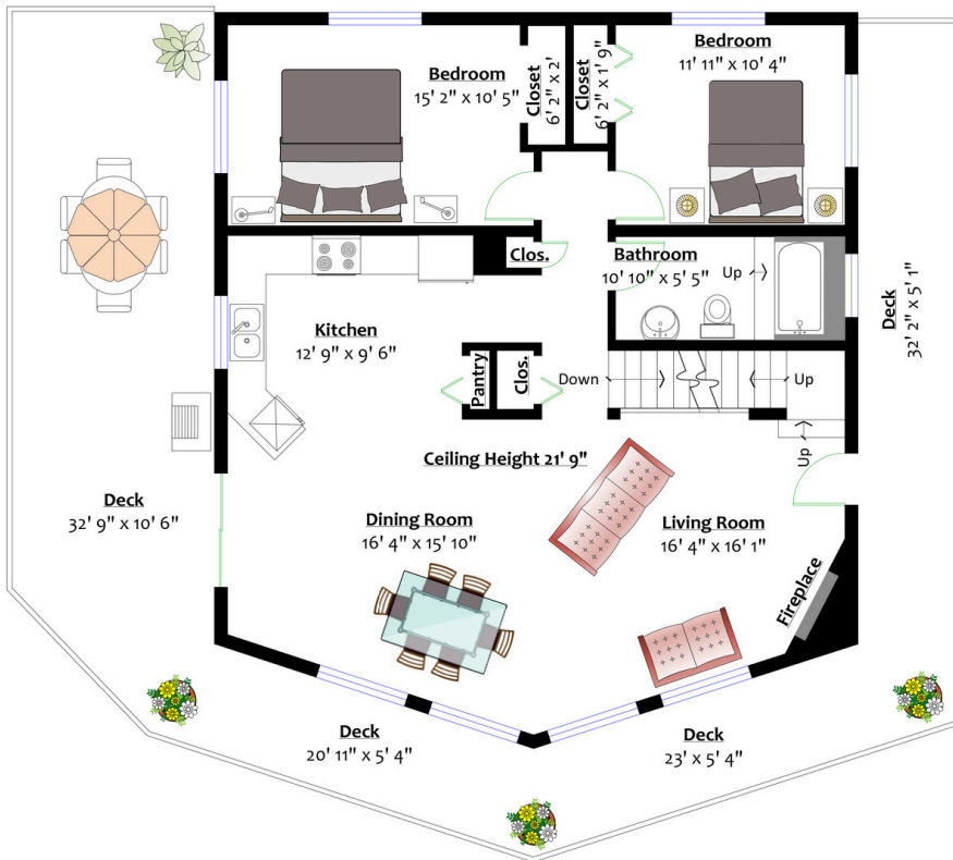
MAIN LEVEL Floor Area: 1,180 Sq. Ft. Ceiling Height: 8'
