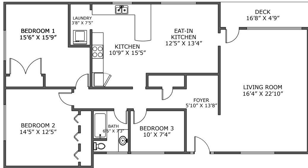
MAIN LEVEL
