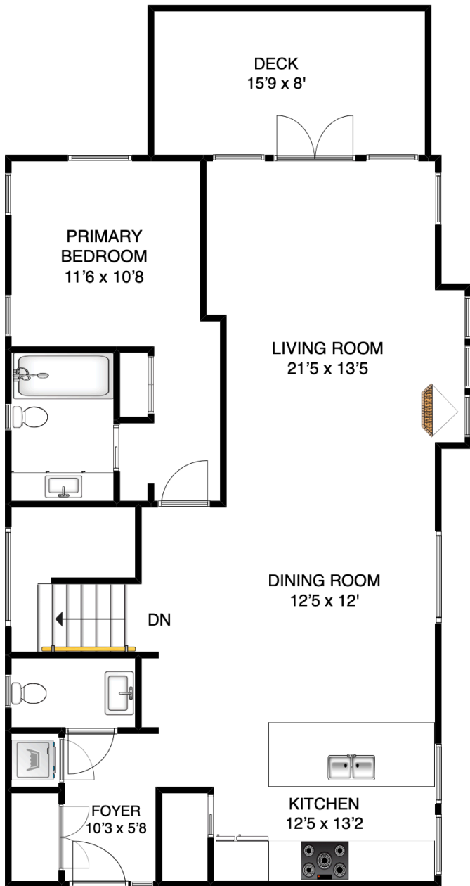
MAIN LEVEL
